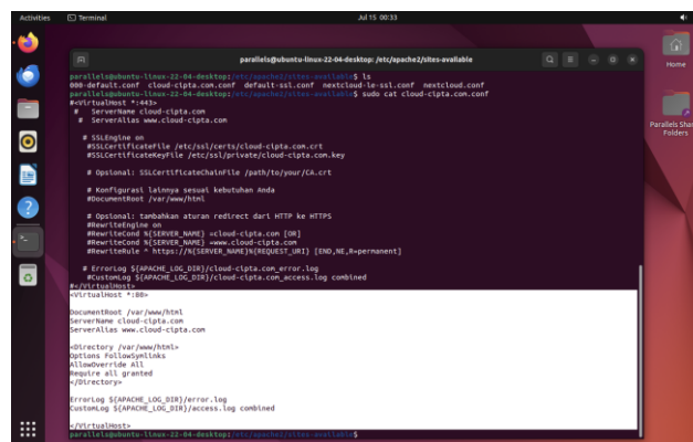
Gambar 9. Proses Penambahan Server Name
